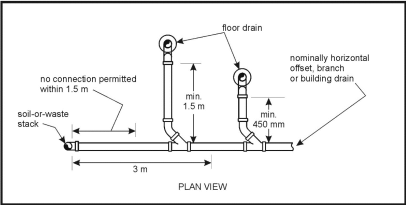
Figure A-2.4.2.1.(5) Soil-or-Waste Pipe Connections
