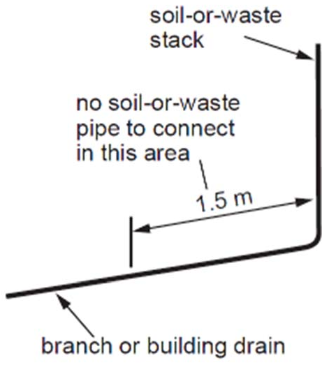
Figure A-2.4.2.1.(4) Soil-or-Waste Pipe Connections
