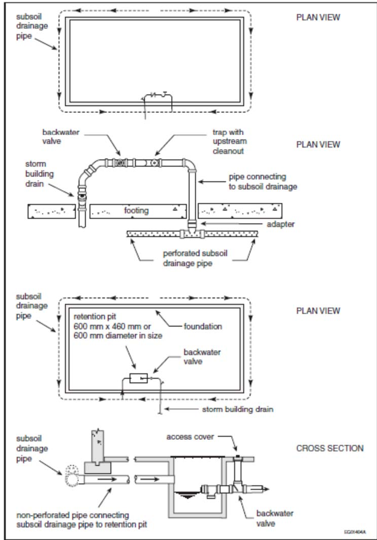
Figure A-2.4.5.3.(1) Subsoil Drainage Connections
