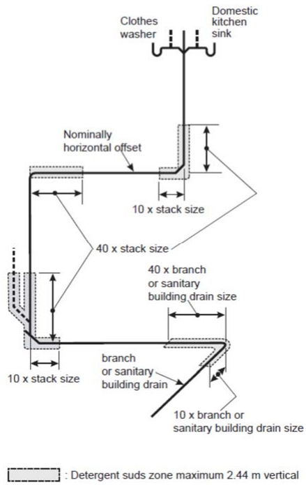
Figure A-2.4.2.1.(6) and (7) Suds pressure zones
