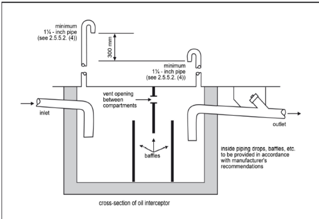
Figure A-2.5.5.2. Venting of Oil Interceptors
