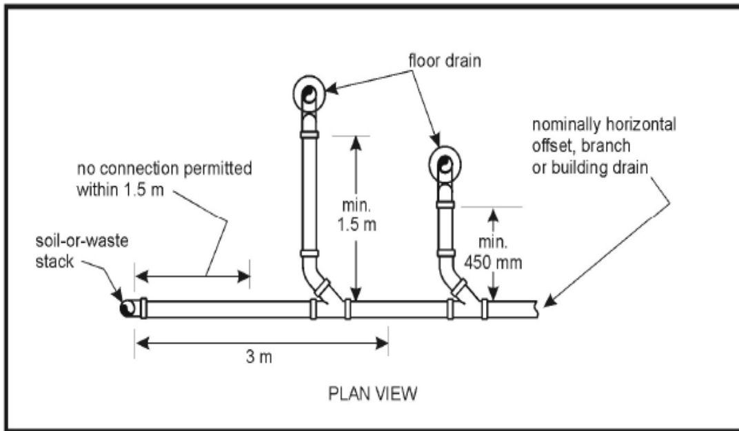
Figure A-2.4.2.1.(5) Soil-or-Waste Pipe Connections
