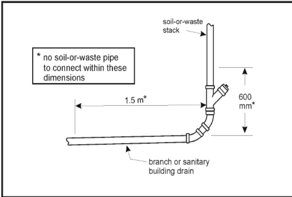
Figure A-2.4.2.1.(4) Soil-or-Waste Pipe Connections
