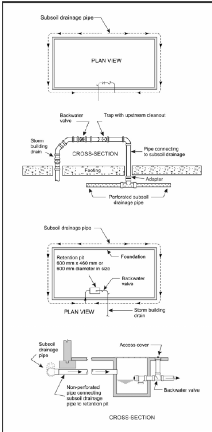
Figure A-2.4.5.3.(1) Subsoil Drainage Connection
