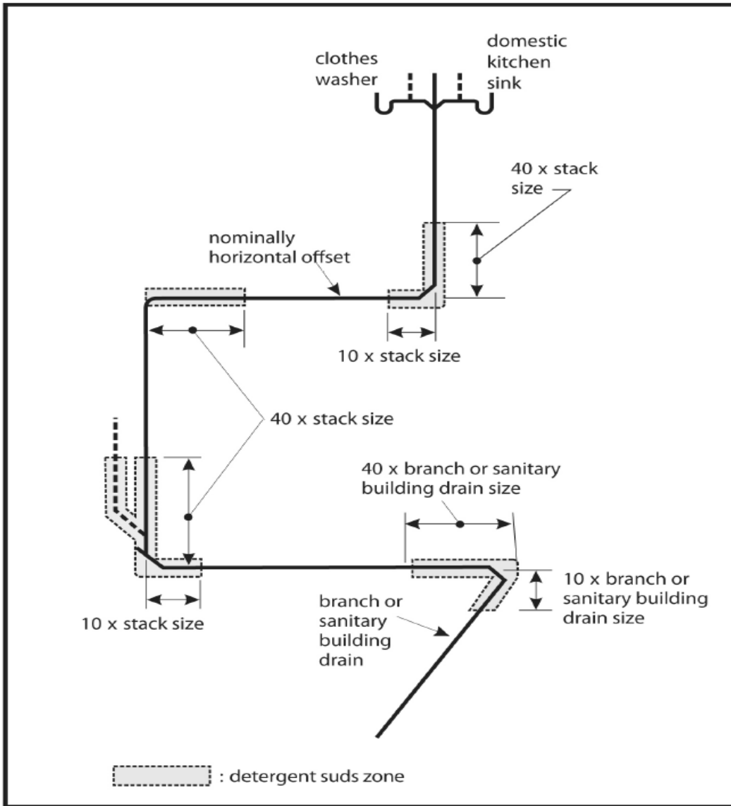
Figure A-2.4.2.1.(6) and (7) Suds pressure zones
